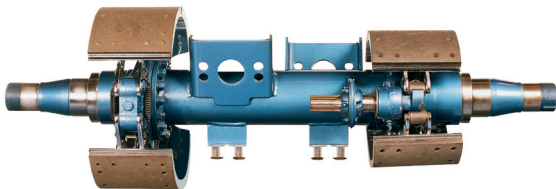
Trunnion/Stubby
