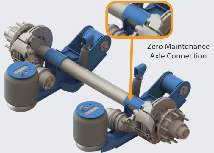
Disc Brake Application
